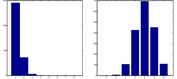
Figure 4: To the left a histogram over the number of solutions with the right orientation and to the right a histogram over the number of real solutions for about 1800 simulated cases.
