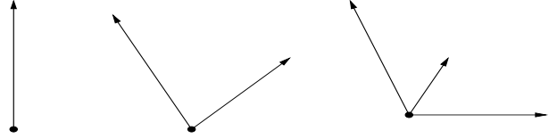
Figure 1: Quivers with one, two and three directions.
