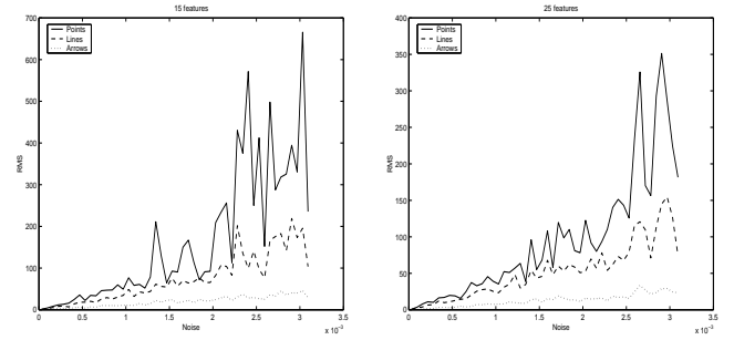
Figure 3: Reprojection error for motion estimated using points (solid), lines (dashed) and 2-quisers (dotted) for 15 features to the left and 25 features to the right.
