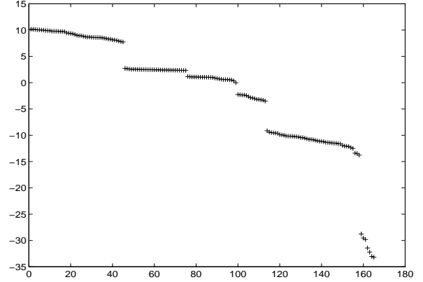
Figure 1: The logarithm of the singular values of the Hessian, A^T A/2 .
