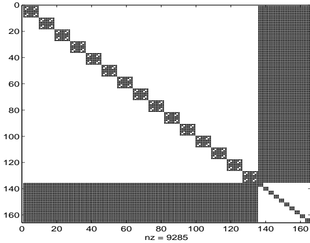
Figure 2: The figure illustrates the structure of the Hessian, A^T A/2 . The nonzero components are shown as black dots in the figure.
