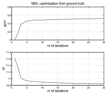
Figure 3: Gcm and DL plotted over number of iterations.
