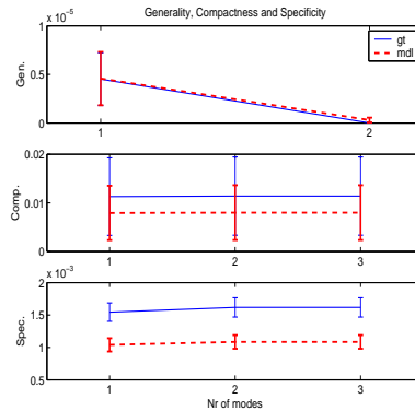
Figure 4: The standard measures of the ground truth and the dl box bump model.
