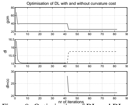
Figure 9: Optimisation of DL and DL + Cur for 4 silhouettes.
