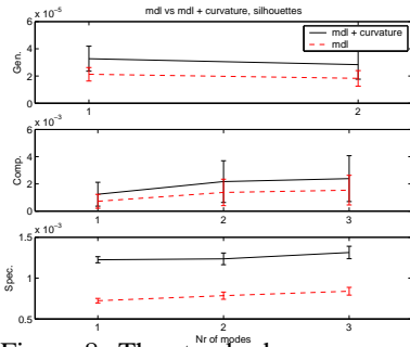
Figure 8: The standard measures of the DL and DL + Cur silhouette model.
