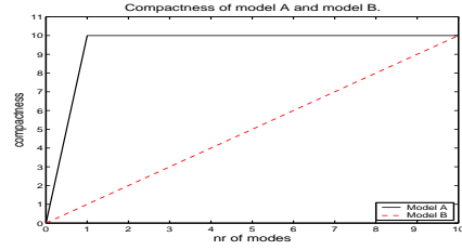
Figure 2: Problem with the compactness measure.
