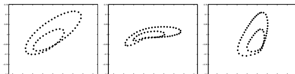
Figure 3. Image curves together with backprojected curve.
