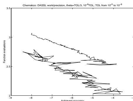
Figure 6.3: Newton termination criteria and computational stability. An ODE was solved using DASSL. Original termination criterion for the Newton iteration is TOL/3 and yields the lower work/precision graph. When the termination criterion is tightened to 10^{-8}TOL (in practice full precision), the upper graph is obtained. It displays a significantly improved computational stability. Work increase, in terms of f evaluations, is moderate (approximately a factor of 2).
