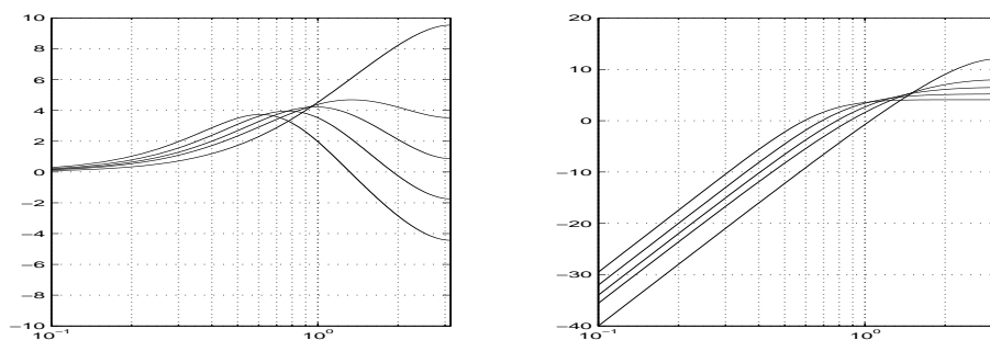
Figure 5.2: Closed loop frequency response. Stepsize frequency response 20 \log^{10} |k \cdot H_{\hat{\varphi}}^0(e^{i\omega})| (left) and error frequency response 20 \log^{10} |G_{\hat{\varphi}}^0(e^{i\omega})| (right) for frequencies \omega \in [0.1, \pi] . From top to bottom at \omega = \pi the graphs are, in both diagrams: PC11 deadbeat; PC.6.9; PC.5.8; PC.4.7; PC.3.6 control. The PC11 has nearly +10 dB amplification of (-1)^n stepsize oscillations (left diagram, \omega = \pi ). Only the PC.4.7 and PC.3.6 controllers attenuate such oscillations; having poles of larger modulus, they are both slower and smoother. G_{\hat{\varphi}}^0(q) contains a double (or second order) difference operator, see (5.11). As a consequence |G_{\hat{\varphi}}^0(e^{i\omega})| = O(\omega^2/(kk_E)) as \omega \rightarrow 0 , causing the 40 dB/decade slopes characteristic of second order adaptivity, at the low frequency end of the error response graphs (right diagram). By contrast, a PI controller’s single integral action only results in first order, 20 dB/decade slopes, see Fig. 4.4. A steeper slope implies stronger suppression of low-frequent variations in \log \hat{\varphi} . The error therefore stays closer to the setpoint \varepsilon = \theta \cdot \text{TOL} .
