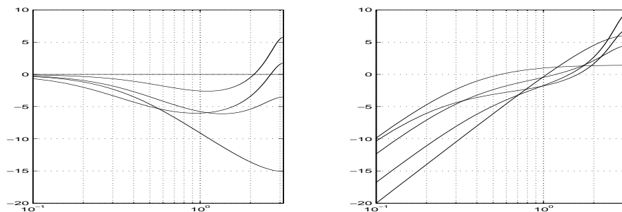
Figure 4.4: Closed loop frequency response . Frequency response is commonly measured in dB and plotted in log-log diagrams, here for frequencies \omega \in [0.1, \pi] . The left diagram shows stepsize frequency response 20 \log^{10} |k \cdot H_{\hat{\varphi}}^0(e^{i\omega})| . The scaling factor k is included to make the response depend only on (kk_I, kk_P) . The right diagram shows the error frequency response 20 \log^{10} |G_{\hat{\varphi}}^0(e^{i\omega})| . From top to bottom at \omega = \pi the graphs are, in both diagrams: PI.68.32; PI.3.4; dead-beat; PI.4.2; PI.3.0 control. The left diagram shows that only the PI.4.2 and PI.3.0 attenuate (-1)^n stepsize oscillations ( -3.5 dB and -15 dB, respectively, at \omega = \pi ); by contrast the PI.68.32 has a significant amplification (almost +6 dB, or a factor of 2) of such oscillations. The purely integrating low-gain controller PI.3.0 is strongly averaging (smoothing) and may be suitable for stochastic differential equations, where \log \hat{\varphi} has a significant high frequency content. The right diagram shows that |G_{\hat{\varphi}}^0(e^{i\omega})| = O(\omega/(kk_I)) as \omega \rightarrow 0 , demonstrating the PI controller's first order adaptivity, see the order conditions in Section 4.3.
