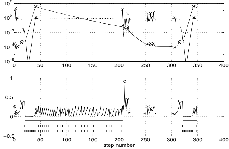
Figure 6.2: Interaction of iteration and stepsize strategies. The upper diagram shows stepsize h and error excess r/\text{TOL} when solving a stiff van der Pol problem; r/\text{TOL} is kept very close to \theta = 0.8 . The lower diagram shows convergence rate \alpha and how it is affected by the strategy described in Section 6. When \alpha is likely to exceed the maximum, the strategy forces either a Jacobian reevaluation or an iteration matrix refactorization, without convergence failures. Jacobian evaluations are indicated by the upper tick marks, matrix refactorizations by the lower tick marks. Solid line indicates Newton iterations; during nonstiff phases, fixed-point iterations were used. During most of the stiff phase (steps 40–205), convergence rate slows down due to a changing Jacobian. By contrast, when the stepsize is increased after passing the turning point (steps 320–345), refactorizations are often necessary, but the same Jacobian can be kept. There is a total of 4% rejected steps (marked \times ) and 1.5% convergence failures (all during nonstiff phase, marked \circ ) in the computation. From [6].
